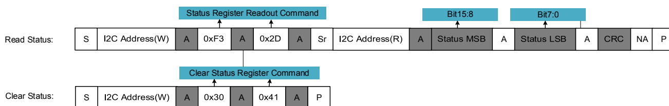
Figure 17 Read Status & Clear Status Sequence
