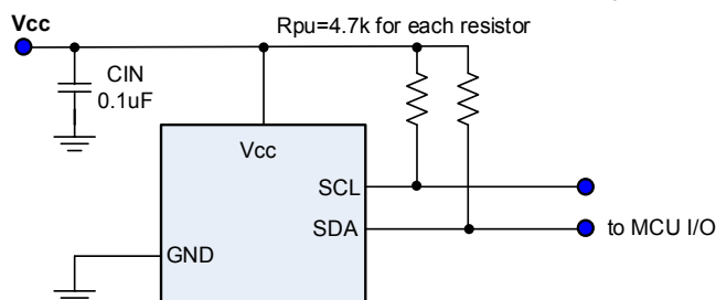
Figure 23 Sensor typical application
