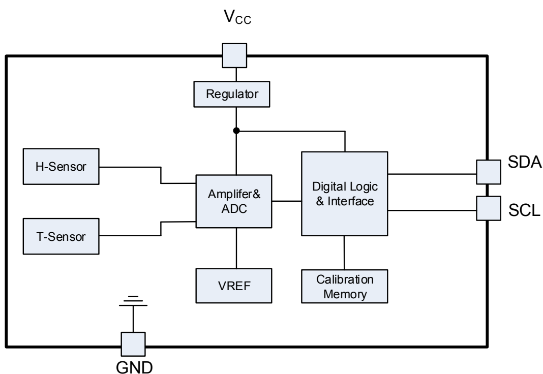
Figure 2 CHT8320 function block
